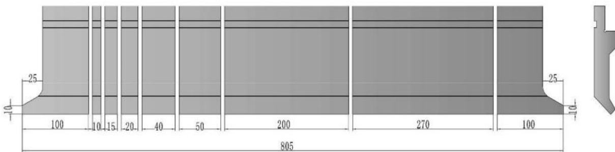
805mm sectioned
